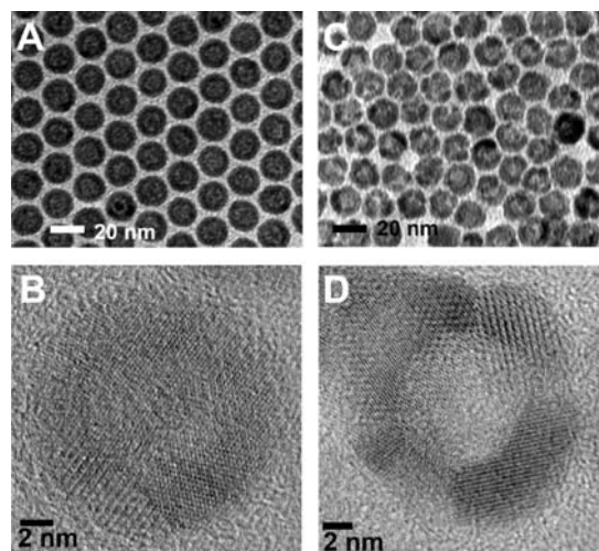
Figure 1. (A) TEM image of the 16 nm HNP of \text{Fe}_3\text{O}_4 . (B) HRTEM image of a single HNP. (C) TEM image of the 16 nm PHNP of \text{Fe}_3\text{O}_4 . (D) HRTEM image of a single PHNP.
